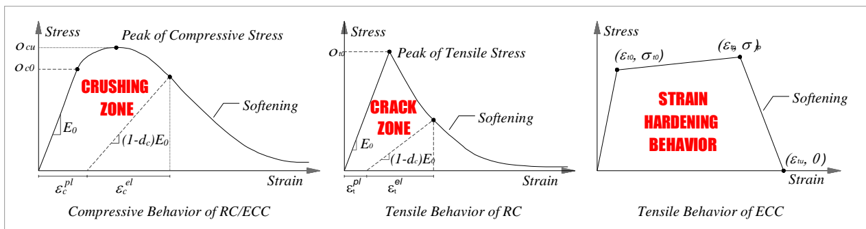
Fig. 3 CDP model for compression and tension
