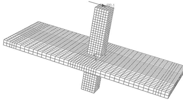
Fig. 2 Finite element mesh of the specimen model.
