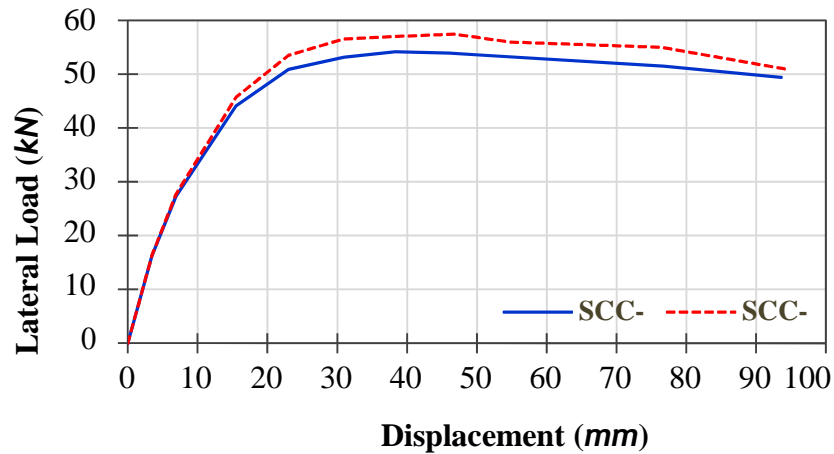
Fig. 4 Load-displacement response of specimens.
